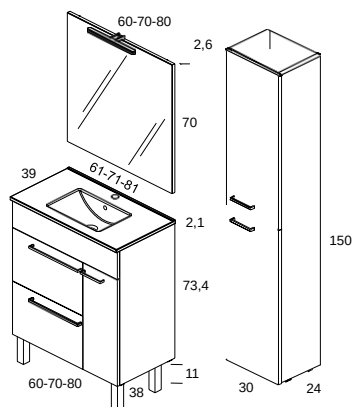
CONFORT C0049955 Columna 30 F-24 · 2P
