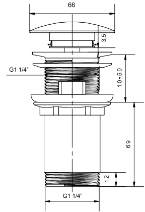
Válvula clic-clac N. 2 Bronce. Ref. 123402
