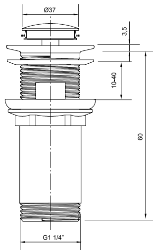
Válvula clic-clac N. 3. Ref. 123403
