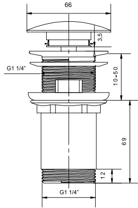
Válvula clic-clac N. 1. Ref. 123401
