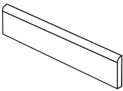
Rodapié Canto Romo Skirting bullnose 8 x 45 cm (3,2" x 18") 8 x 60 cm (3,2" x 24") 8 x 90 cm (3,2" x 36")
