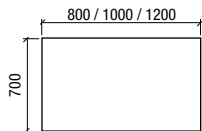
Espejo TOULOUSE 1200 horizontal luz led (20 W) IP 44 1200 x 700 mm
